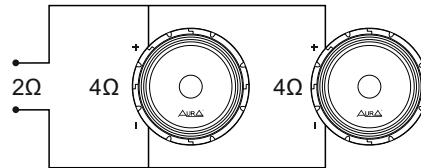
Parallel connection
