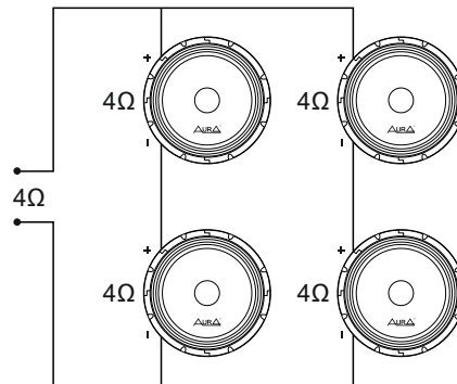
Serial-parallel connection
