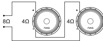
Serial connection
